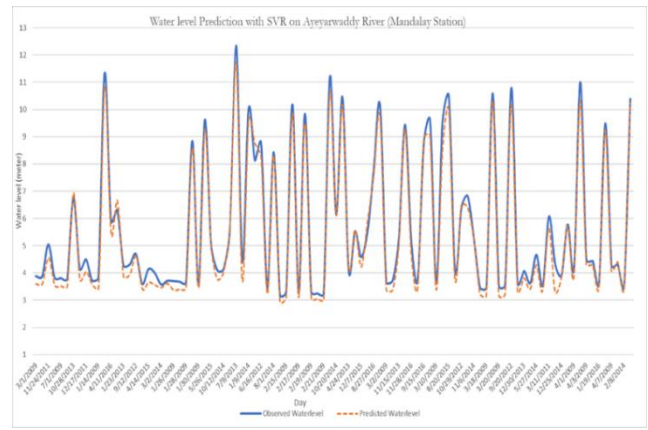
Figure 2. Predicted 5 lead day water levels of Mandalay station by SVR
