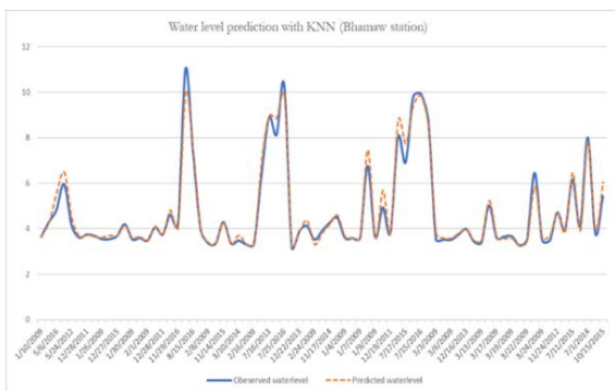
Figure 1. Predicted 5 lead day water levels of Bhamo station by KNN
