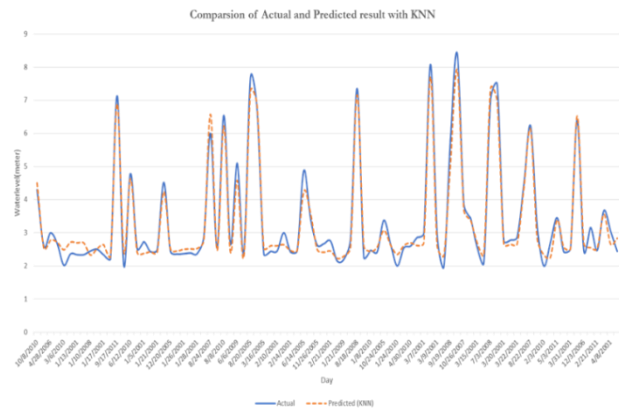
Figure 3. Predicted 5 lead day water levels of Bago station by KNN
