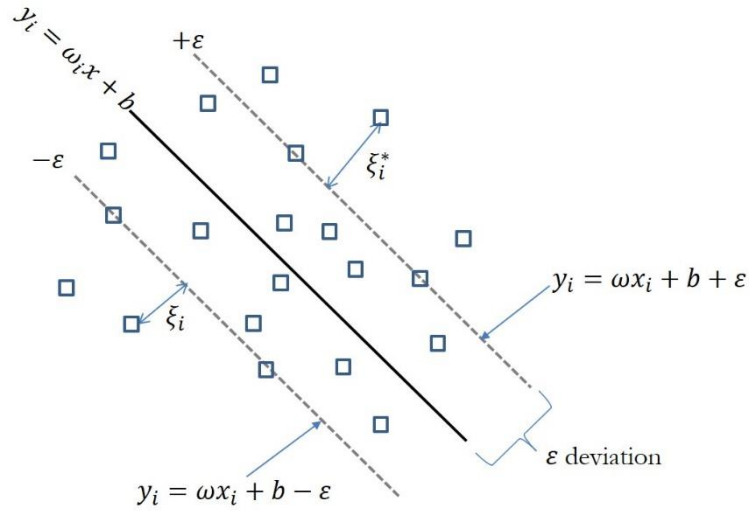
Figure 3.4. Illustration of \epsilon tube with slack variable and data point
